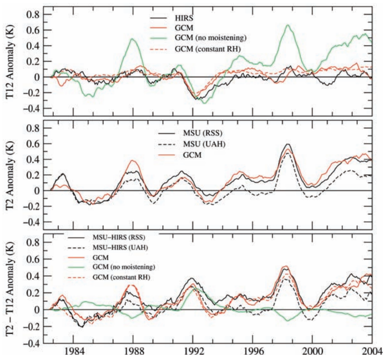
Fig. 2. Global mean time series of T12 (top), T2 (middle), and T2 – T12 (bottom) from GCM simulations (red) and satellite observations (black). The model-simulated radiances are also shown from calculations using a seasonally varying climatological profile with no moistening trend [green line (21)] and a prescribed moisture profile that moistens at a constant relative humidity rate [red dashed line (21)]. All time series are smoothed with a 6-month running mean.
