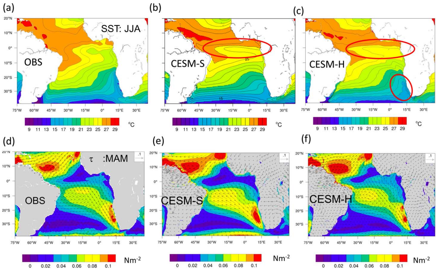
Figure 11. Climatological Mean SST for June-July-August (JJA): from (a) Levitus/WOA98, (b) CESM-S, and (c) CESM-H. Corresponding climatological mean wind stress vectors ( \text{Nm}^{-2} ) and magnitude of the mean vectors (color) in March-April-May (MAM) from (d) QuikSCAT observations [Risien and Chelton, 2008], (e) CESM-S, and (f) CESM-H.
