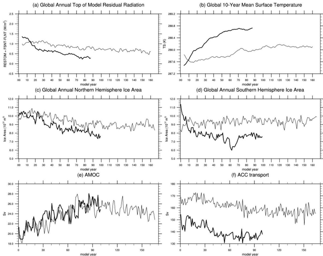
Figure 1. Time series of globally averaged quantities for 100 years of CESM-H (thick black line) and 166 years of CESM-S (thin gray line). (a) Top of atmosphere net radiation, positive incoming to Earth. Data are 10 year running mean. (b) Surface (including ocean, land, ice) temperature, 10 year running average. Sea ice area in (c) Northern Hemisphere and (d) Southern Hemisphere. (e) Atlantic Meridional Overturning Circulation (AMOC), 12 month running averages, (f) transport through Drake Passage due to Antarctic Circumpolar Current (ACC), annual values.
