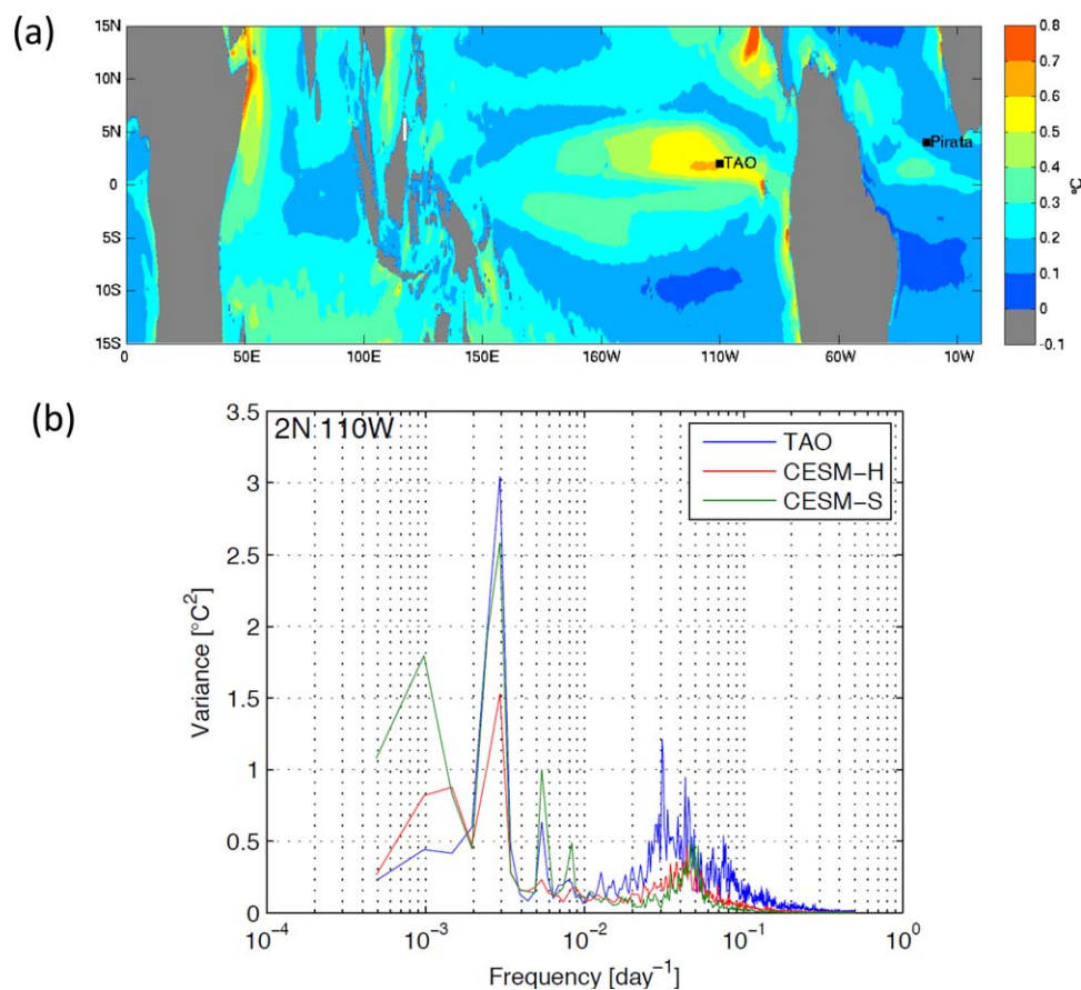
Figure 8. (a) SST standard deviation from CESM-H data filtered to show sub-90 day variability. Squares show locations of a Tropical Atmosphere Ocean (TAO) mooring at 110°W, 2°N and a PIRATA mooring at 23°W, 4°N. (b) Variance spectra of unfiltered daily SST at location of TAO mooring, from CESM-H (red), CESM-S (green), and TAO (blue).
