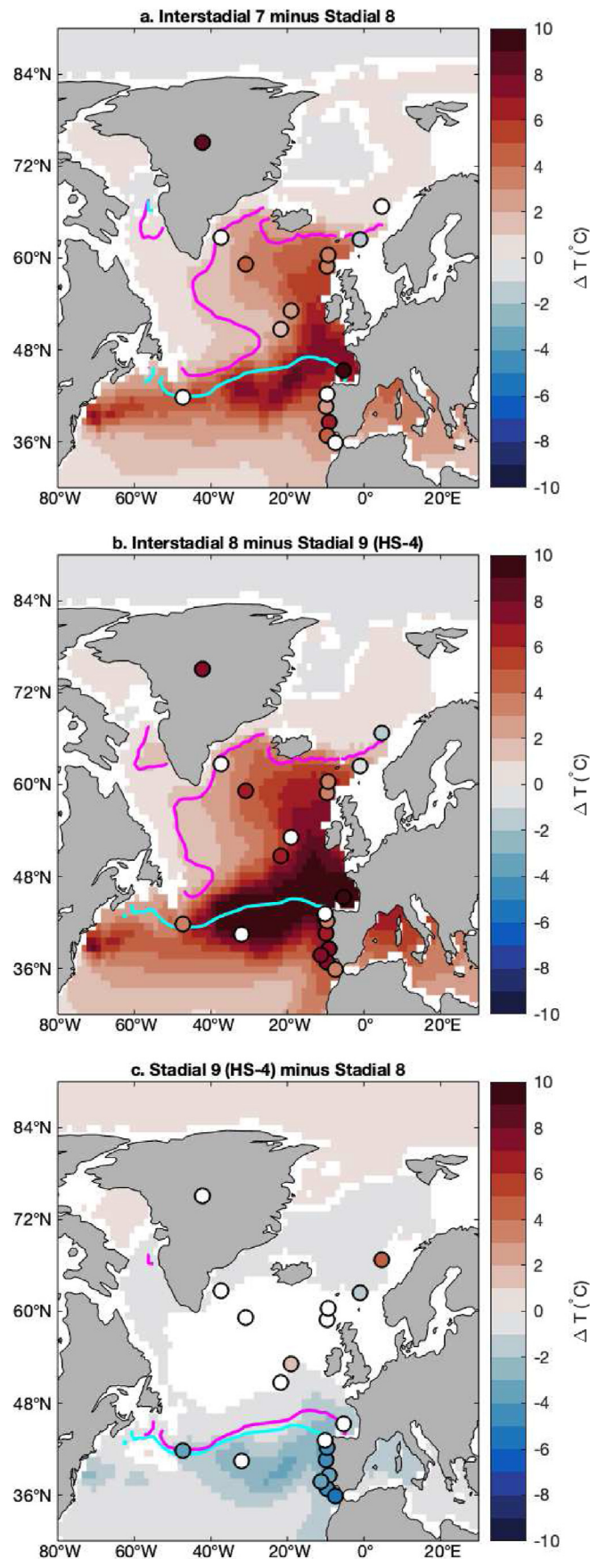
Fig. 5. (Figure previous page). Mapping the summer 10-m temperature differences between climate states in the D-O events in proxy data (points) and in the model (shading). a) Interstadial warming following a non-Heinrich stadial. b) Interstadial warming following a Heinrich stadial. c) The additional cooling in a Heinrich stadial compared to a non-Heinrich stadial. In each map, violet and cyan lines mark the model mean summer sea ice extent (15% contour) for the warmer and cooler states respectively. Proxy data are only plotted where there are two or more data points per interval at the core site. Data and model anomalies that are not significant (according to a two-sided Students' t-test at the p < 0.05 level) are filled/shaded white. In calculating the temperature means at each site over the stadials and interstadials, we leave out the first and last 200 years of each interval to reduce sensitivity to dating uncertainty (changing the buffer between 0 and 500 years has little affect on the key patterns, though it does cause the significance of some anomalies to drop from the 95%–90% level). Although proxy data are nominally calibrated to 10-m water depth, the reconstructed temperatures may be representative of greater depths in some locations (see discussion of Nordic Seas sites in the main text). (For interpretation of the references to colour in this figure legend, the reader is referred to the Web version of this article.)
