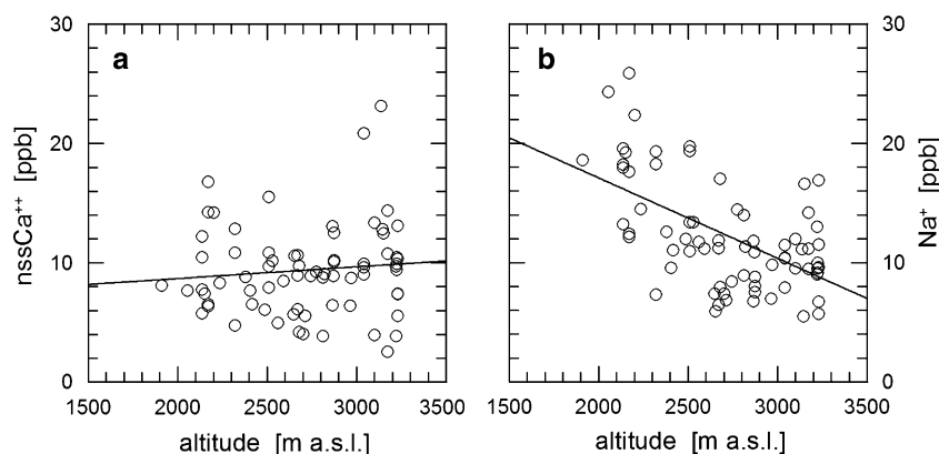
Fig. 7 Altitude dependence of a nss \text{Ca}^{2+} and b \text{Na}^+ concentrations in north to central Greenland snow pits and shallow ice cores (lines are linear regressions). Data are from the AWI North Greenland traverse 1993–1995 (Fischer 1997), the EGIG
