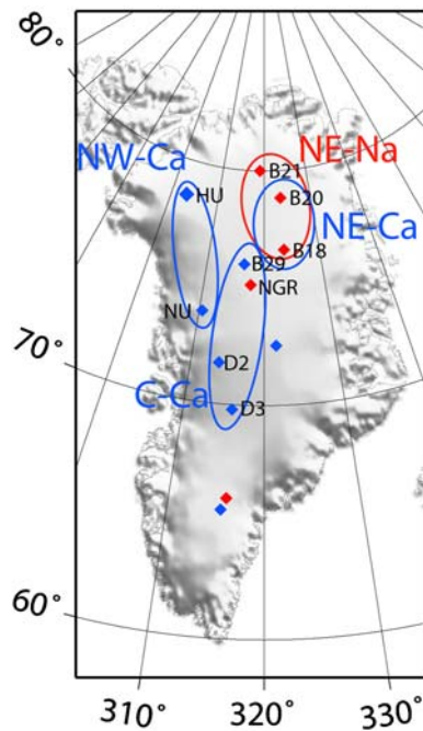
Fig. 1 Map of the Greenland ice core records. In red are cores where both, \text{Ca}^{2+} and \text{Na}^+ records were available, blue only \text{Ca}^{2+} . Named cores were selected for the four regional groups resulting from the EOF analysis (see Sect. 2). The four groups, which were subsequently used for the regression/validation model, are also depicted
